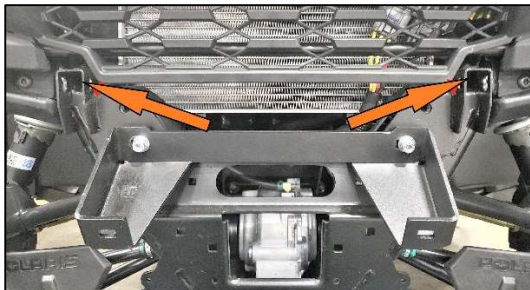
Figure 8: Stock Bumper Mounting Location
