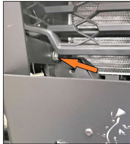
Figure 10: Bumper Mounting Bolt Inside
